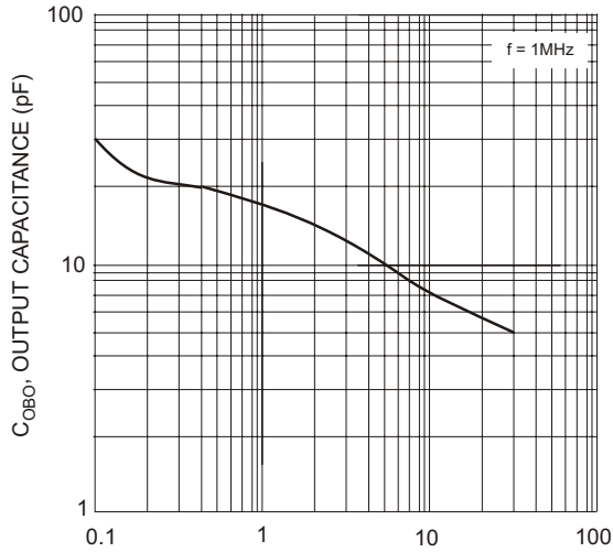
Fig. 3, Output Capacitance vs. Collector-Base Voltage
